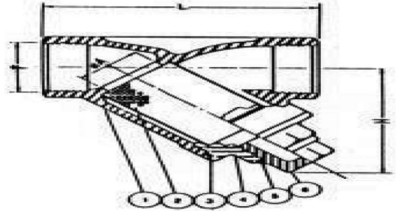
AK-8210 Y-TYPE STRAINERS, SCREW ENDS MATERIAL: S.S. 316 INVESTMENT CASTING SIZE: 1/4" THRU 4"
